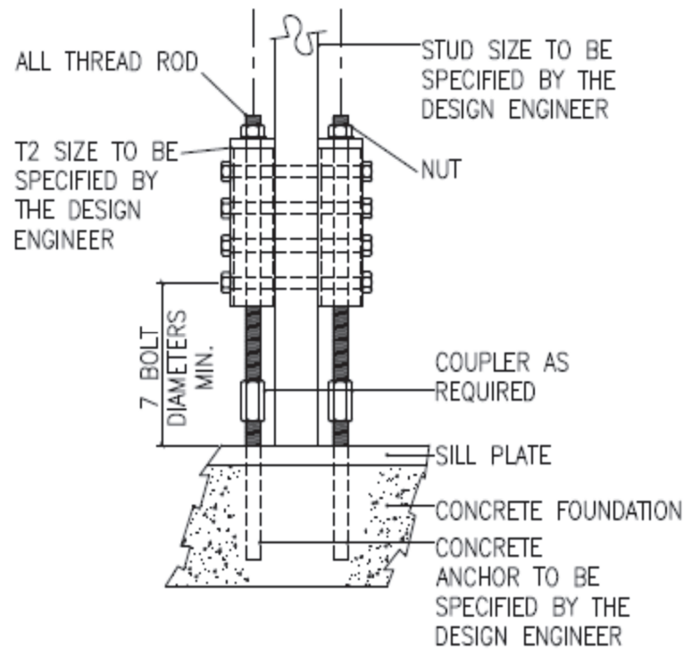
FIGURE 3—PAIRED CONNECTION
