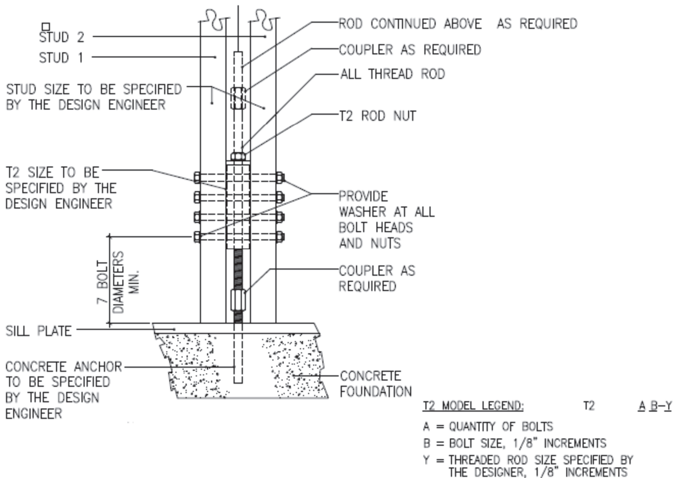
FIGURE 4—SANDWICH CONNECTION
